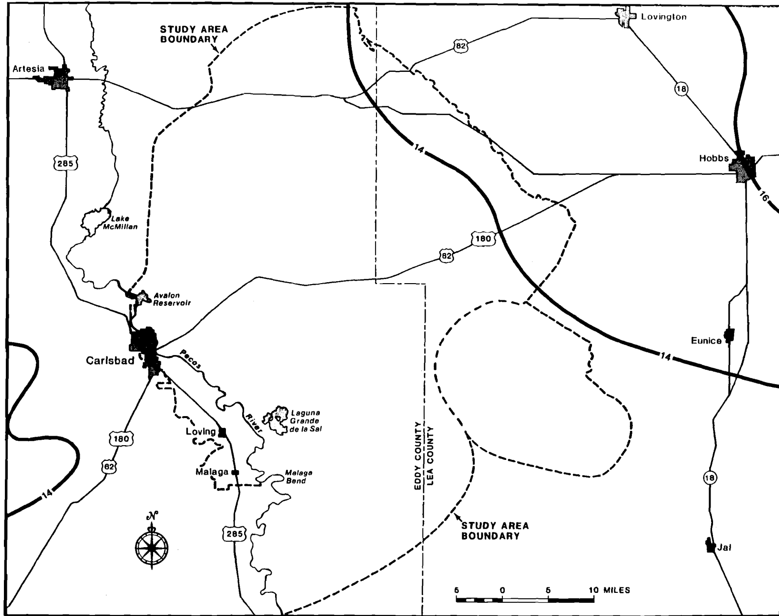
(c) Contours Published by the New Mexico State Planning Office (Tuan and others, 1973) Figure 3. (Concluded)
